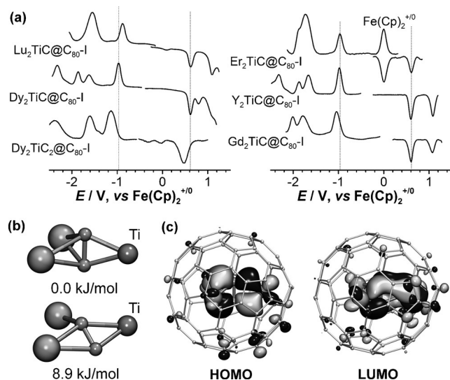
Figure 3. a) Square-wave voltammetry of \text{M}_2\text{TiC}@C_{80}\text{-I} ( \text{M} = \text{Lu}, \text{Dy}, \text{Er}, \text{Y}, \text{Gd} ) and \text{Dy}_2\text{TiC}_2@C_{80}\text{-I} measured in o -dichlorobenzene/tetrabutylammonium hexafluorophosphate ( o -DCB/TBAPF 6 ). b) Two conformations of the \text{Lu}_2\text{TiC}_2 cluster in the DFT-optimized molecular structure of \text{Lu}_2\text{TiC}_2@C_{80}\text{-I} (atoms are shown as spheres with the radius decreasing from Lu to Ti to C). c) HOMO and LUMO of \text{Lu}_2\text{TiC}_2@C_{80}\text{-I} computed at the PBE/TZVP level.
