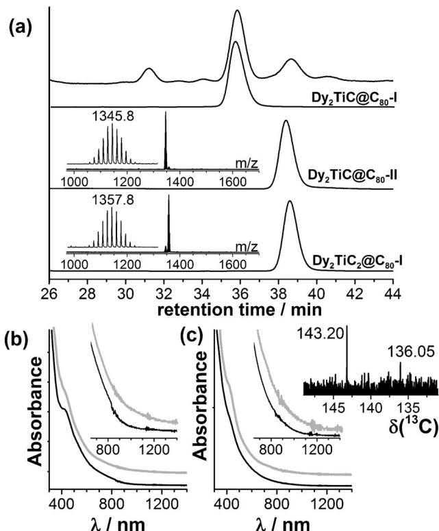
Figure 4. a) HPLC trace of the raw Dy-Ti extract (top) and HPLC curves for individual \text{Dy}_2\text{TiC}@C_{80}\text{-I} , \text{Dy}_2\text{TiC}@C_{80}\text{-II} , and \text{Dy}_2\text{TiC}_2@C_{80}\text{-I} ; the insets show their mass spectra. b,c) UV/Vis/NIR absorption spectra of (b) \text{M}_2\text{TiC}@C_{80}\text{-II} and (c) \text{M}_2\text{TiC}_2@C_{80}\text{-I} (black: \text{M} = \text{Dy} , gray: \text{M} = \text{Lu} ); the inset shows the ^{13}\text{C} NMR spectrum of \text{Lu}_2\text{TiC}_2@C_{80}\text{-I} .
