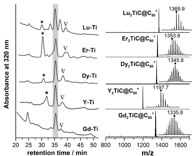
Figure 1. Left: HPLC chromatograms of raw extracts obtained in metal/Ti/CH 4 arc-discharge syntheses (Buckyprep column, toluene as eluent); asterisks mark the fractions with M 3 N@C 80 , shaded rectangle highlights the fractions with M 2 TiC@C 80 -I, whereas triangles denote the fractions with M 2 TiC@C 80 -II/M 2 TiC 2 @C 80 -I. Right: positive-ion MALDI mass spectra of isolated M 2 TiC@C 80 -I; insets show isotopic distributions and mass numbers of the most intense peaks (marked with the dot).
