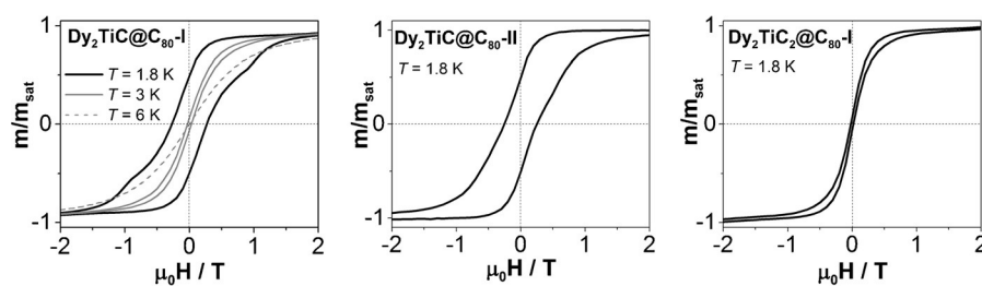
Figure 5. Magnetization curves of \text{Dy}_2\text{TiC}@C_{80}\text{-I} , \text{Dy}_2\text{TiC}@C_{80}\text{-II} , and \text{Dy}_2\text{TiC}_2@C_{80}\text{-I} measured by SQUID. All shown curves are measured at 1.8 K with a sweep rate of 5 \text{ mT s}^{-1} ; for \text{Dy}_2\text{TiC}@C_{80}\text{-I} the measurements at 3 K and 6 K are also shown.
