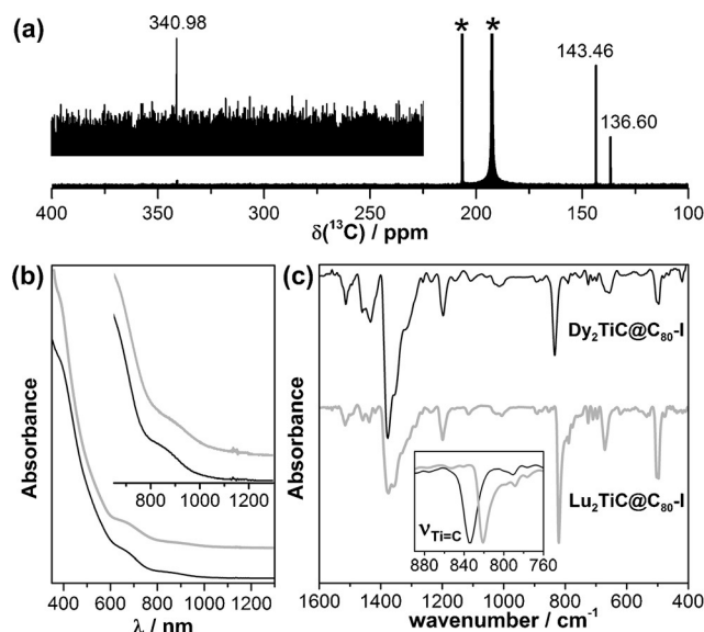
Figure 2. a) 13 C NMR spectrum of 13 C-enriched Lu 2 TiC@C 80 -I, asterisks mark the lines of the solvent and the lock. b) Vis/NIR absorption spectra of M 2 TiC@C 80 -I in toluene. c) FTIR spectra of M 2 TiC@C 80 -I (gray: M = Lu; black: M = Dy). The inset in (c) compares two spectra in the range of the Ti=C stretching mode.
